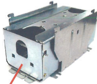
PA192 Slide In Cash Box Assembly (300S)
