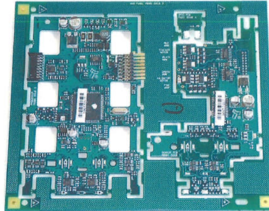
PB185_CNV NV9 Mother Board
